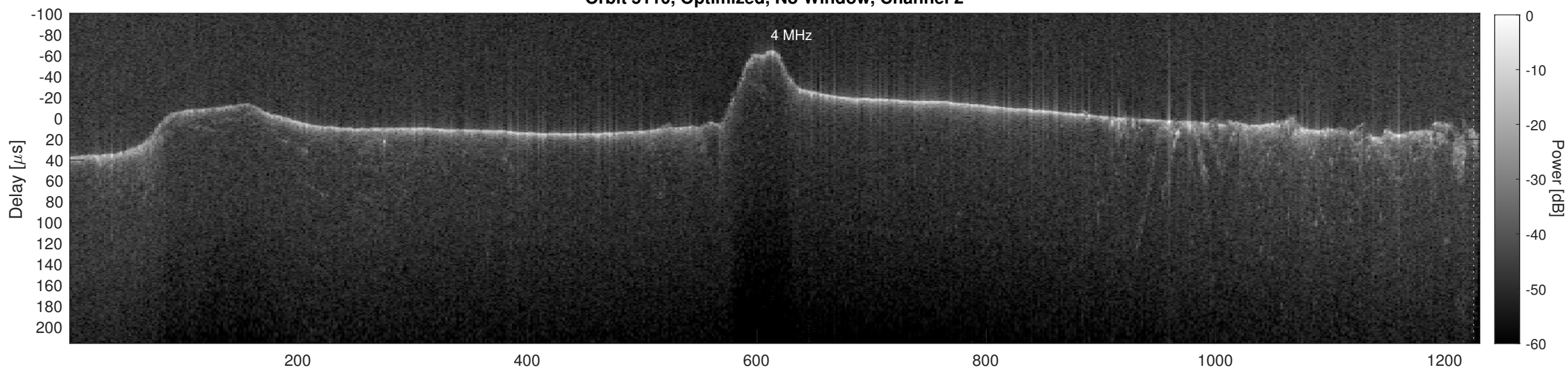
Orbit 5110, Cluttergram
