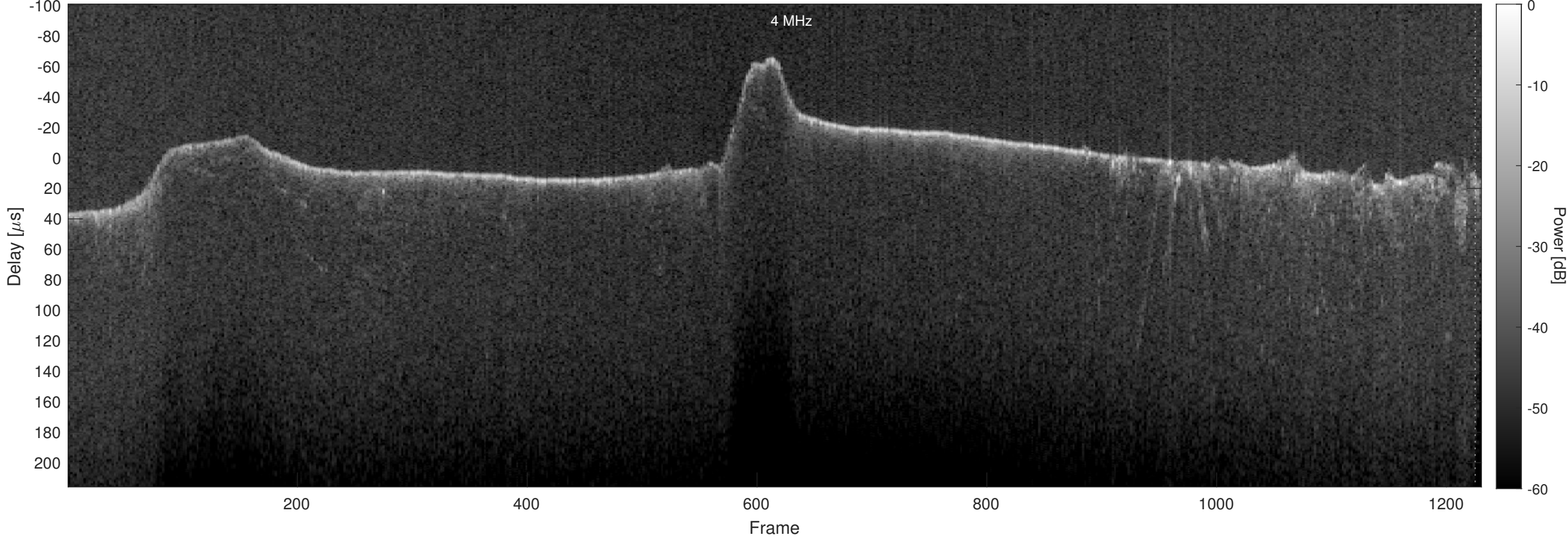
Orbit 5110, Optimized, Window, Channel 2
