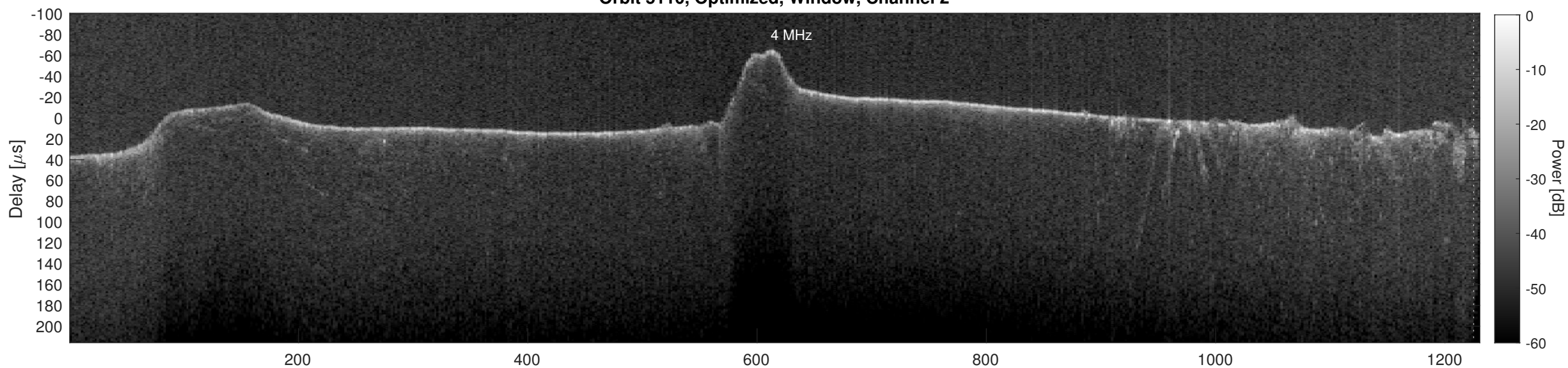
Orbit 5110, Cluttergram
