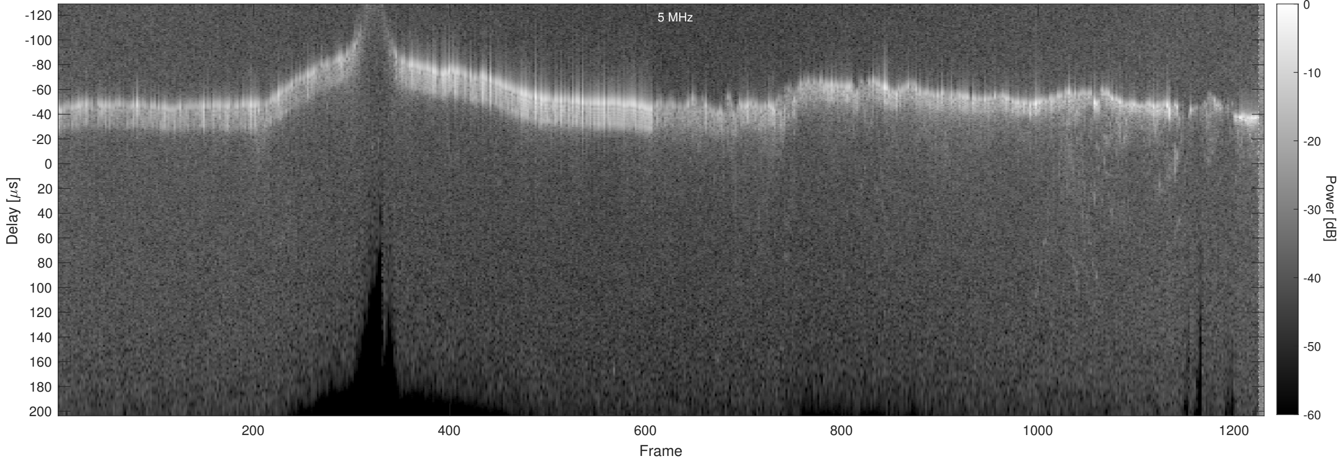
Orbit 5111, Chapman, No Window, Channel 2
