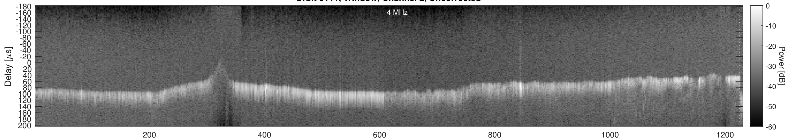
Orbit 5111, Window, Channel 2, Chapman
