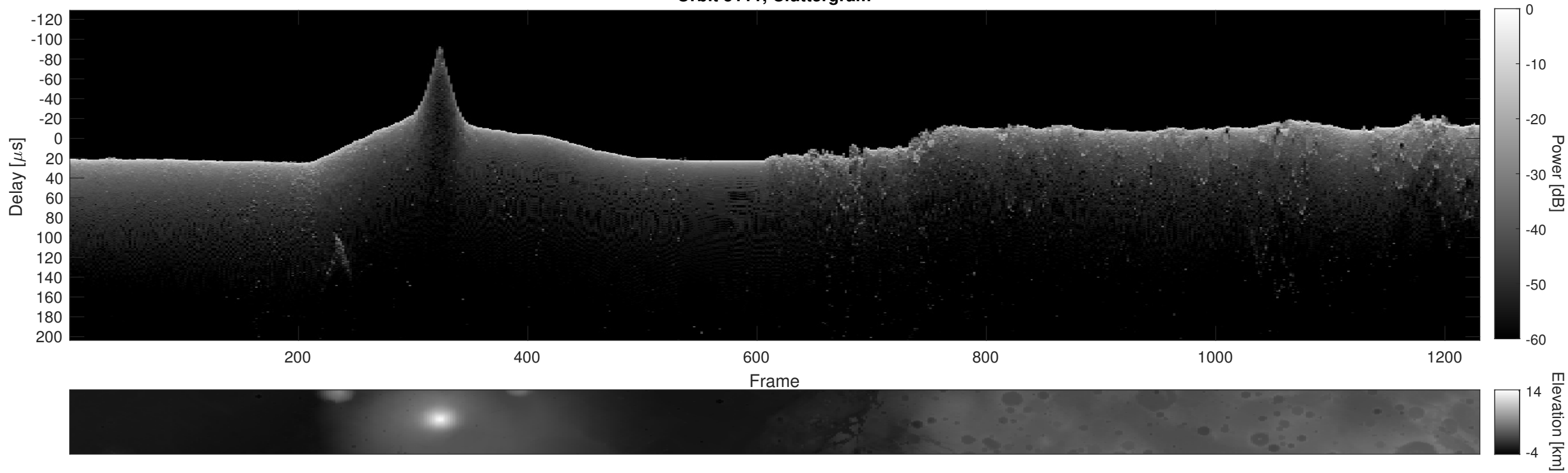
Orbit 5111, Cluttergram
