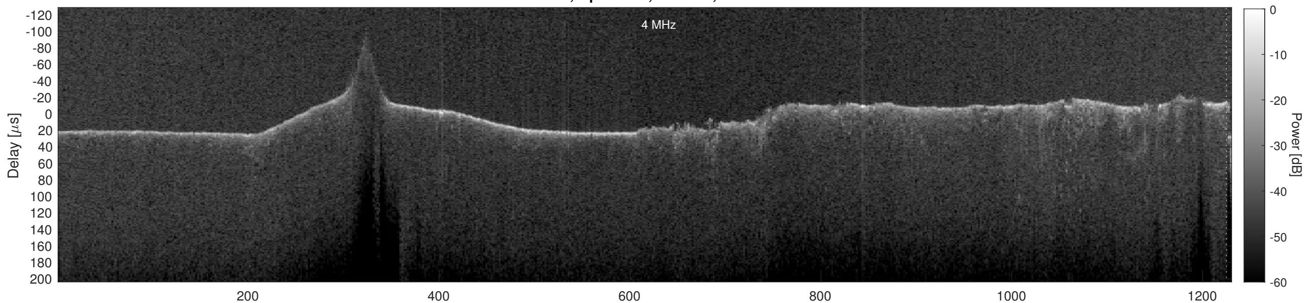
Orbit 5111, Cluttergram
