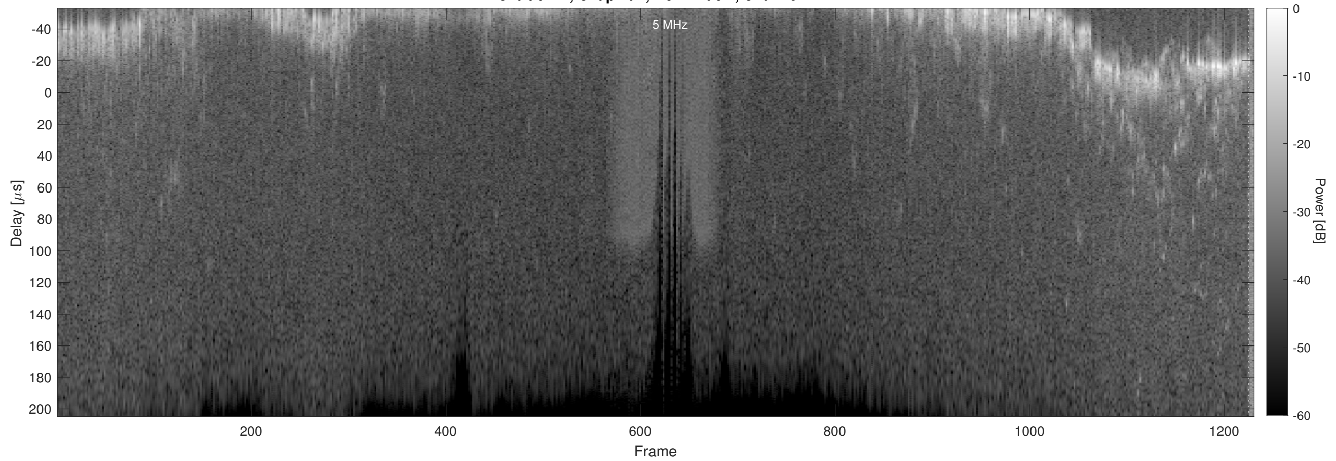
Orbit 5112, Chapman, No Window, Channel 2
