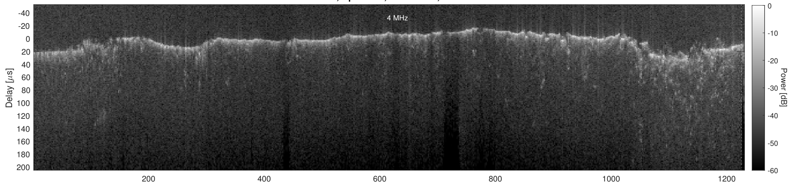
Orbit 5112, Cluttergram
