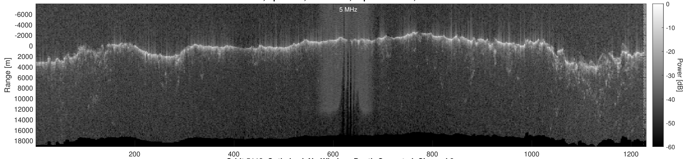
Orbit 5112, Optimized, No Window, Depth-Corrected, Channel 2
