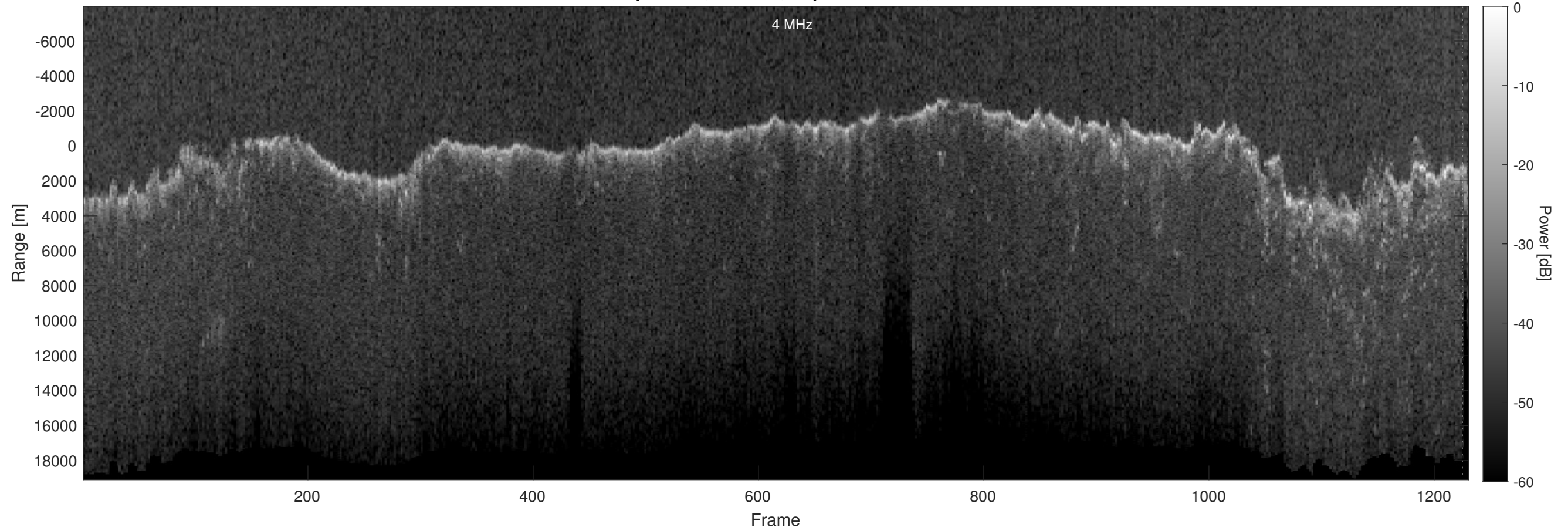
Orbit 5112, Optimized, Window, Depth-Corrected, Channel 2
