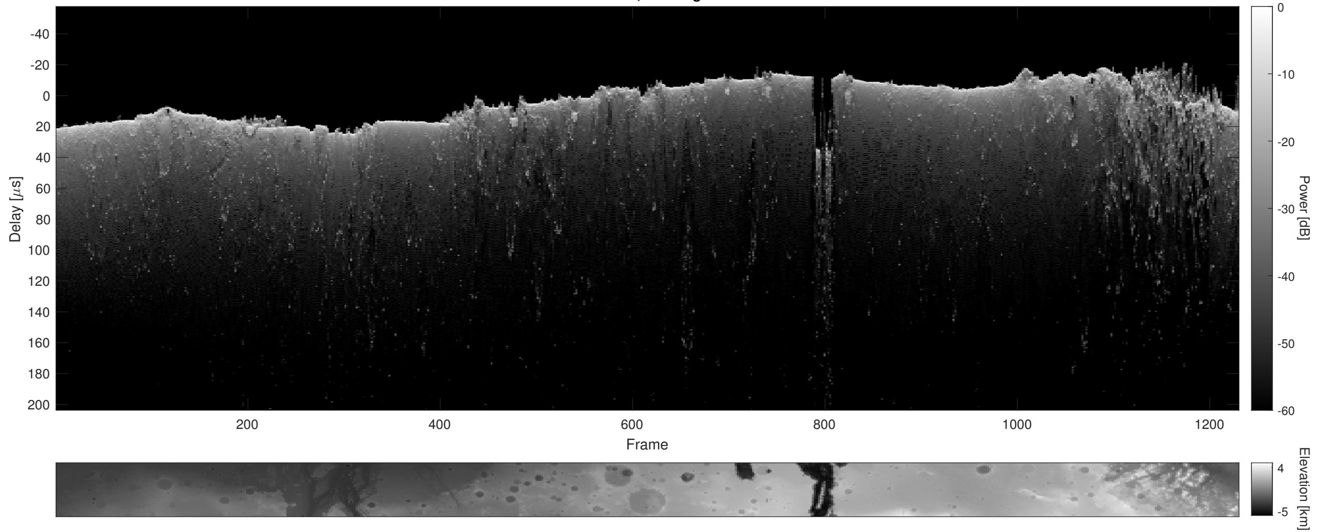
Orbit 5113, Cluttergram
