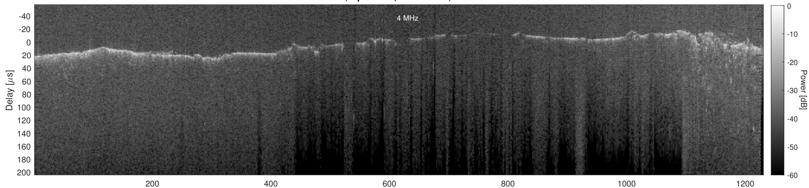
Orbit 5113, Cluttergram
