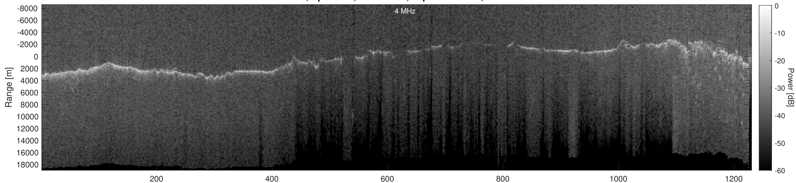
Orbit 5113, Depth-Corrected Cluttergram
