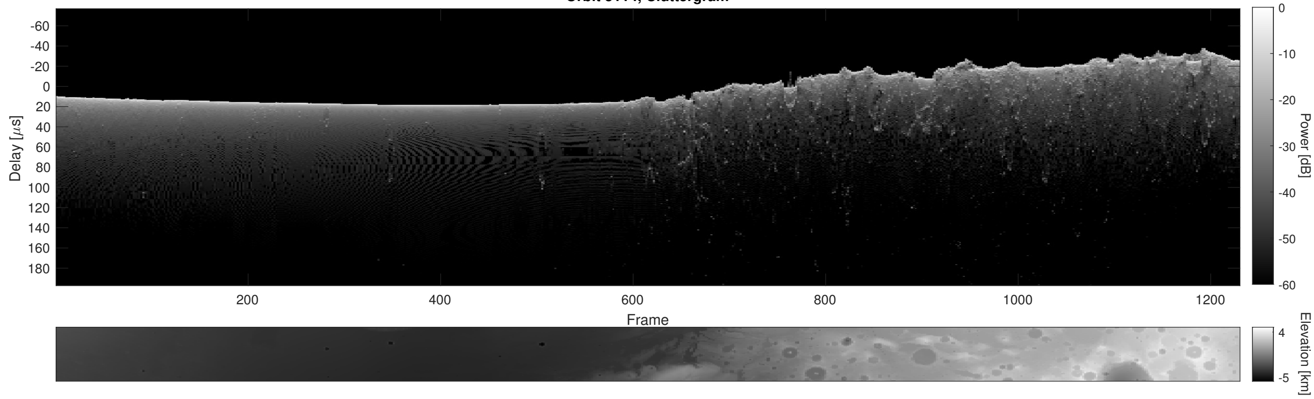
Orbit 5114, Cluttergram
