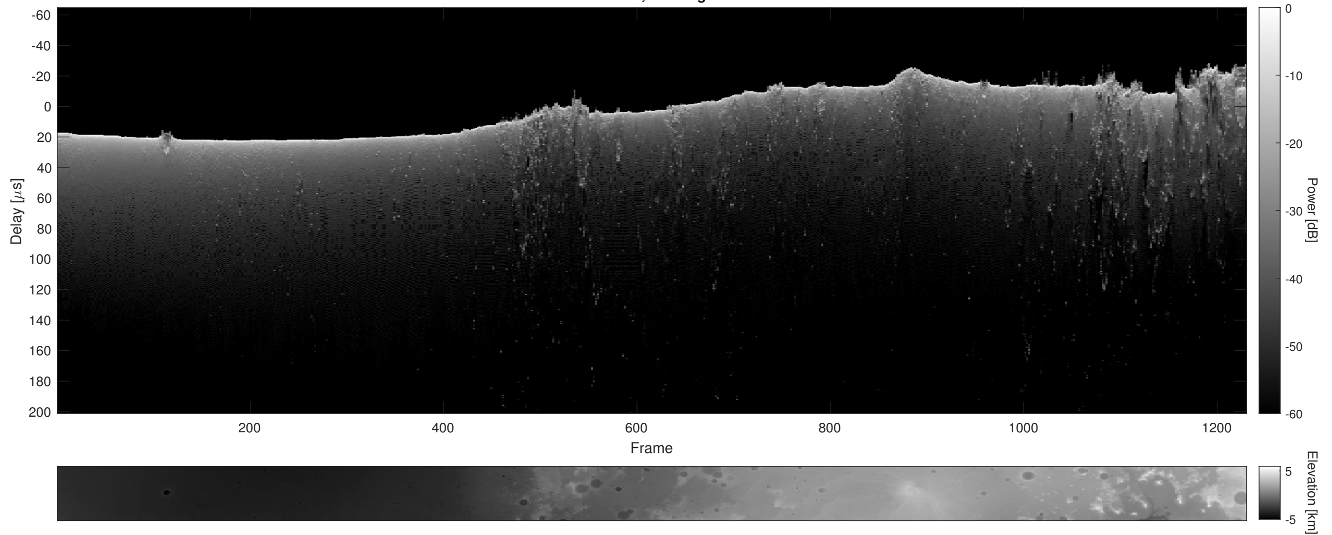
Orbit 5115, Cluttergram
