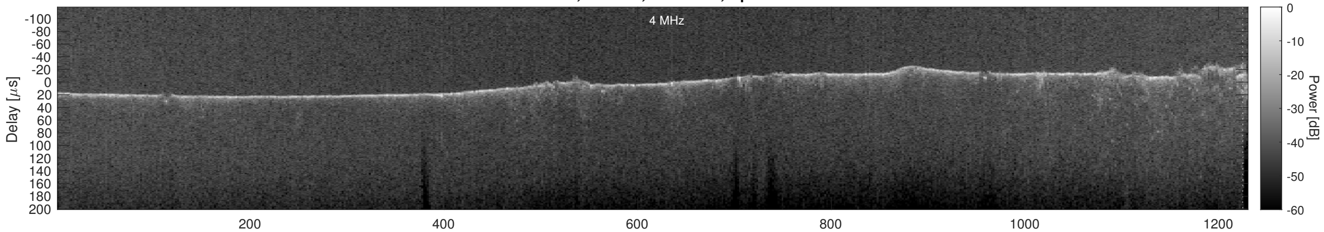
Orbit 5115, Cluttergram
