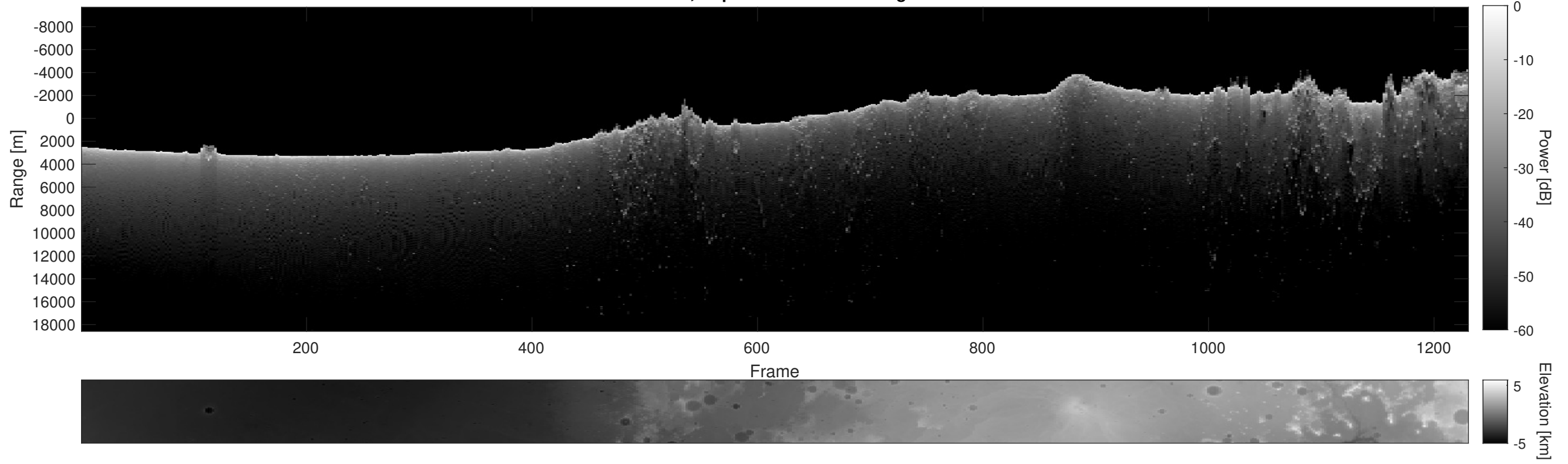
Orbit 5115, Depth-Corrected Cluttergram
