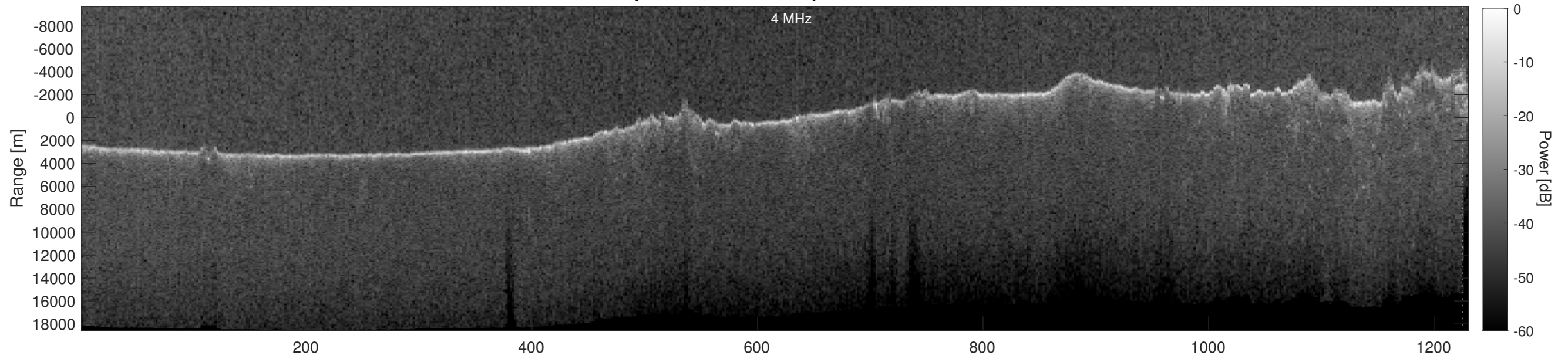
Orbit 5115, Depth-Corrected Cluttergram
