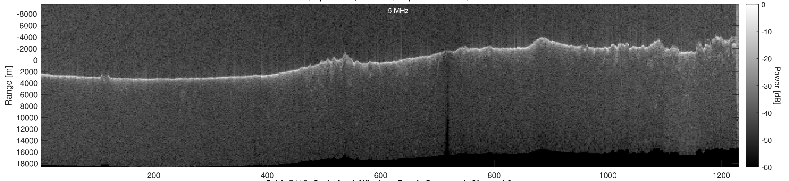
Orbit 5115, Optimized, Window, Depth-Corrected, Channel 2
