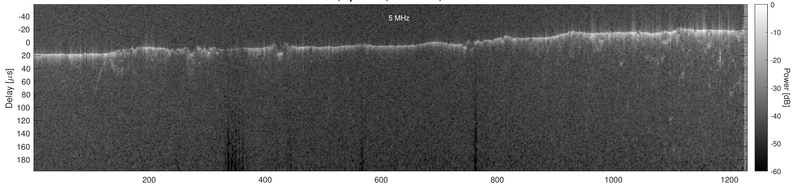
Orbit 5116, Optimized, No Window, Channel 2
