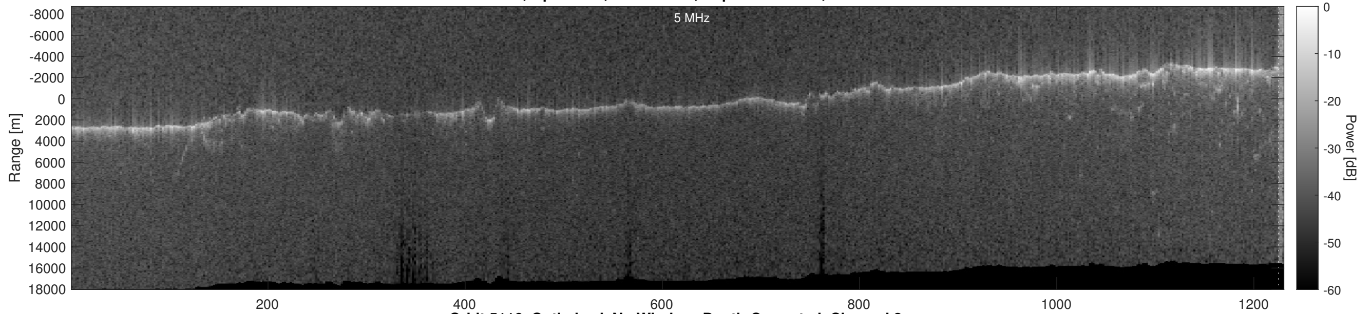
Orbit 5116, Optimized, No Window, Depth-Corrected, Channel 2
