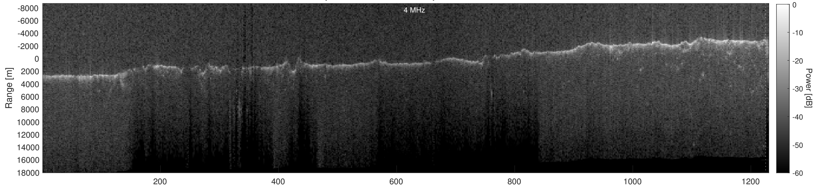
Orbit 5116, Depth-Corrected Cluttergram
