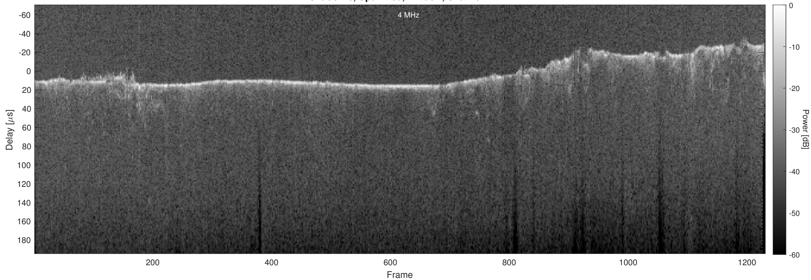
Orbit 5118, Optimized, Window, Channel 2
