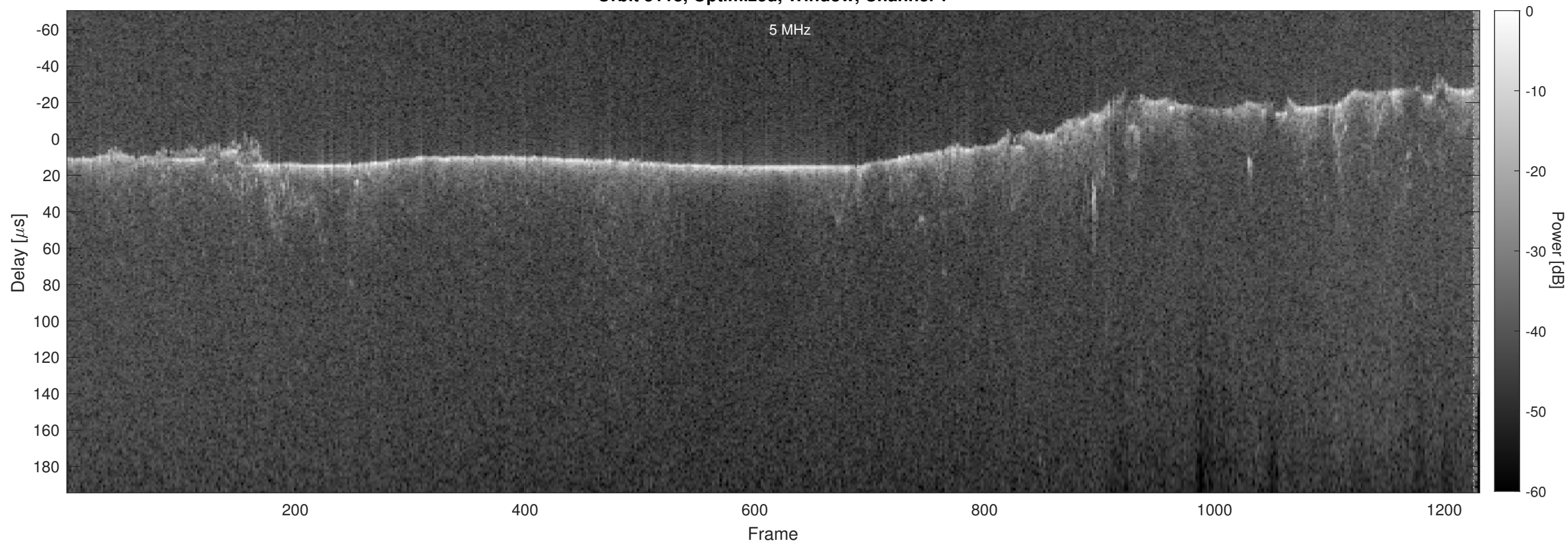
Orbit 5118, Optimized, Window, Channel 2
