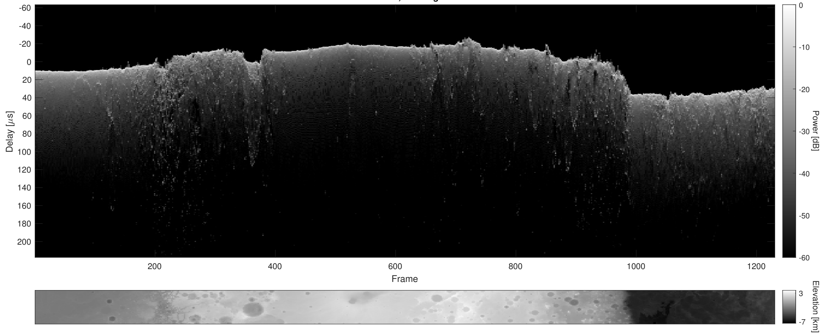
Orbit 5119, Cluttergram
