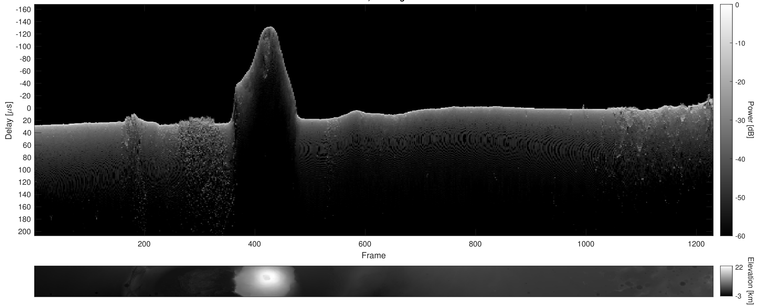
Orbit 5121, Cluttergram
