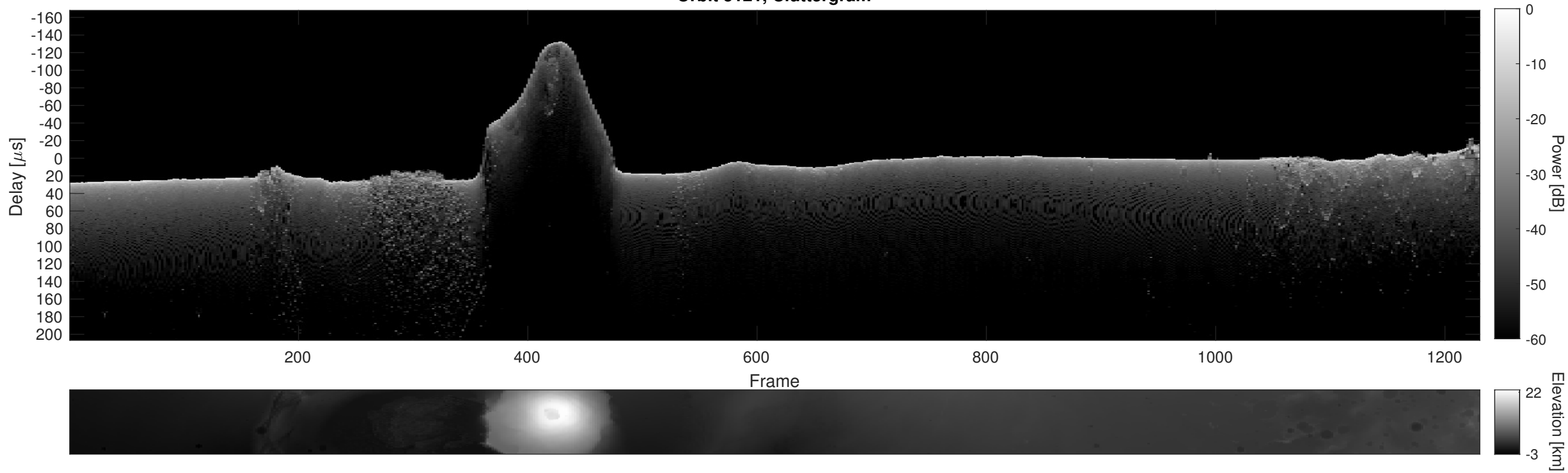
Orbit 5121, Cluttergram
