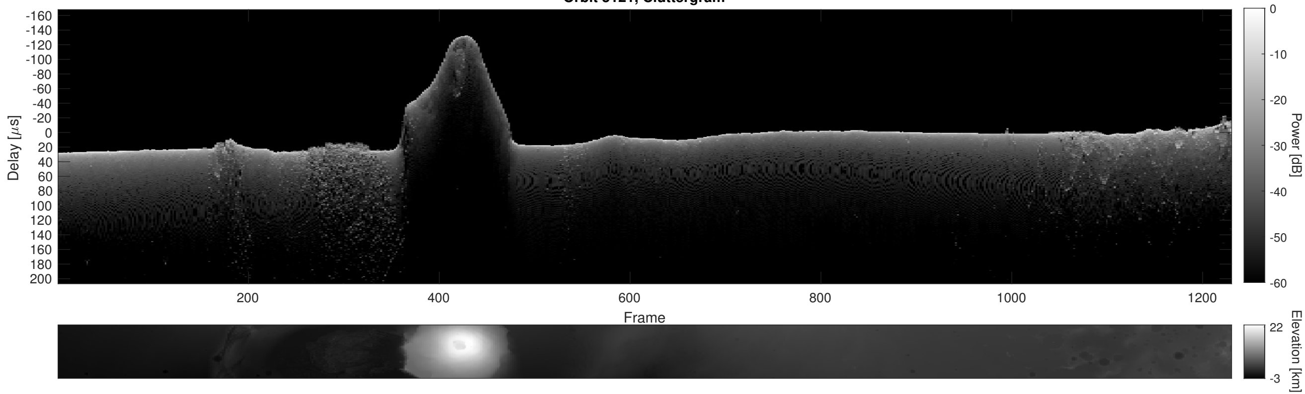
Orbit 5121, Cluttergram
