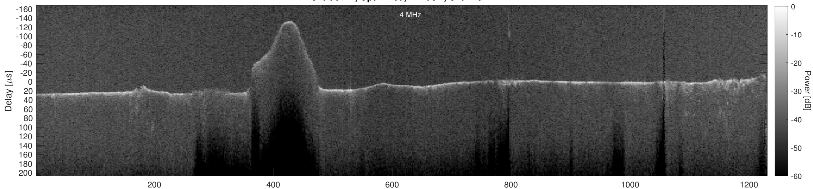
Orbit 5121, Cluttergram
