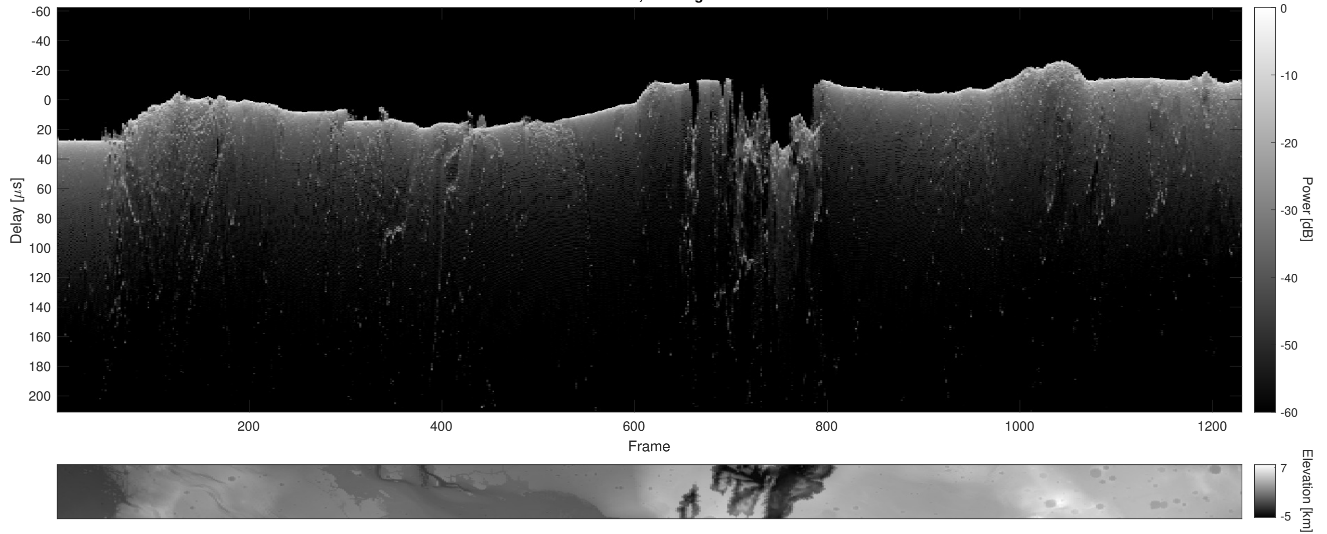
Orbit 5124, Cluttergram
