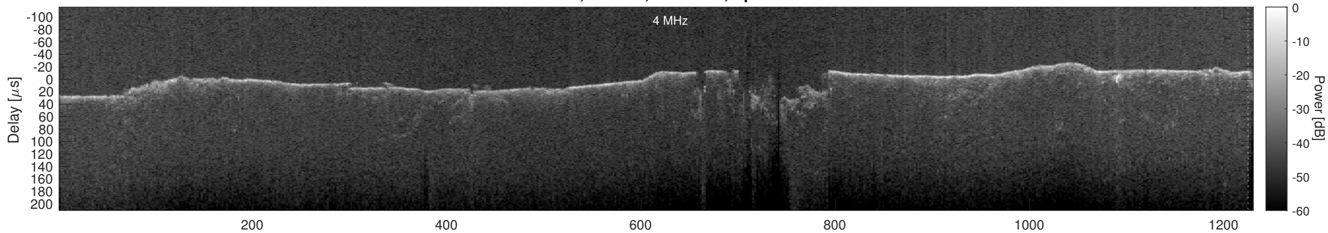
Orbit 5124, Cluttergram
