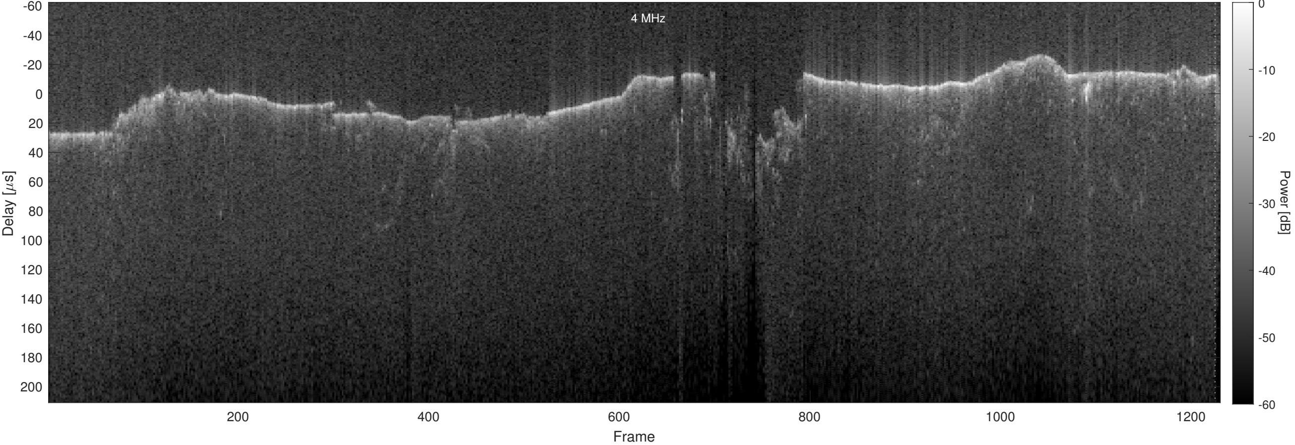
Orbit 5124, Optimized, No Window, Channel 2
