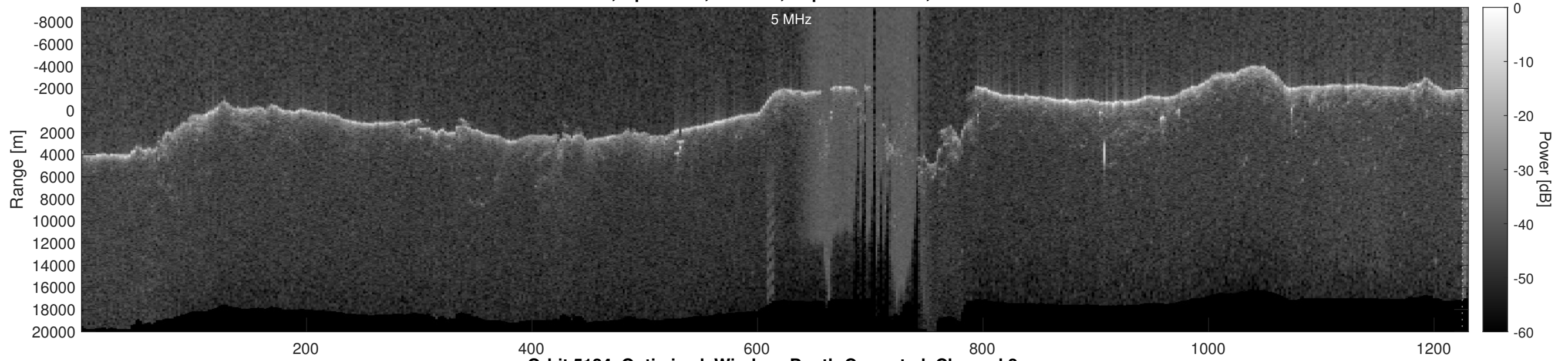
Orbit 5124, Optimized, Window, Depth-Corrected, Channel 2
