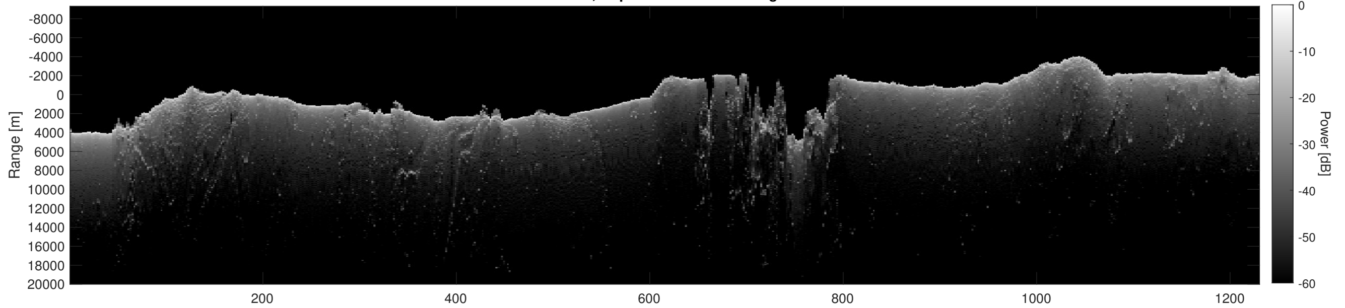
Orbit 5124, Depth-Corrected Cluttergram
