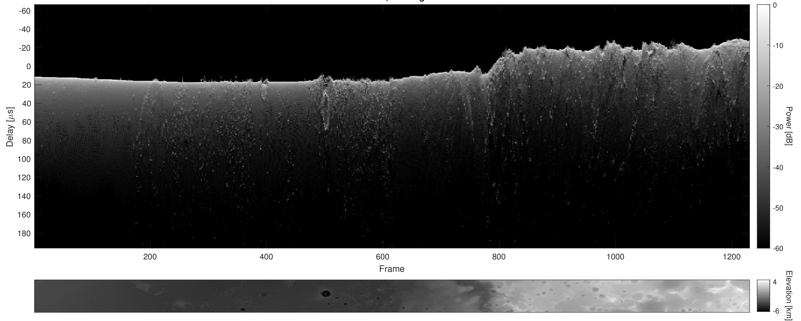
Orbit 5125, Cluttergram
