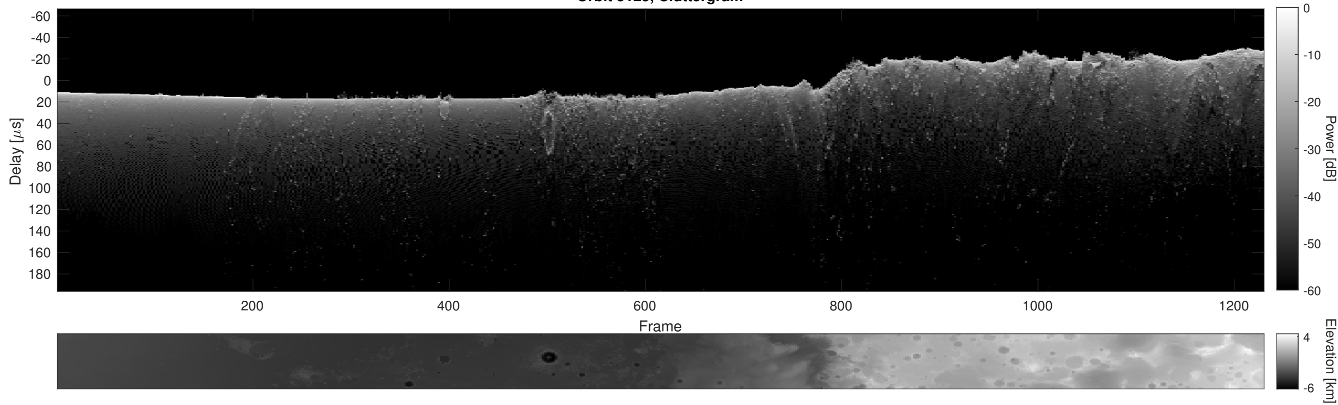
Orbit 5125, Cluttergram
