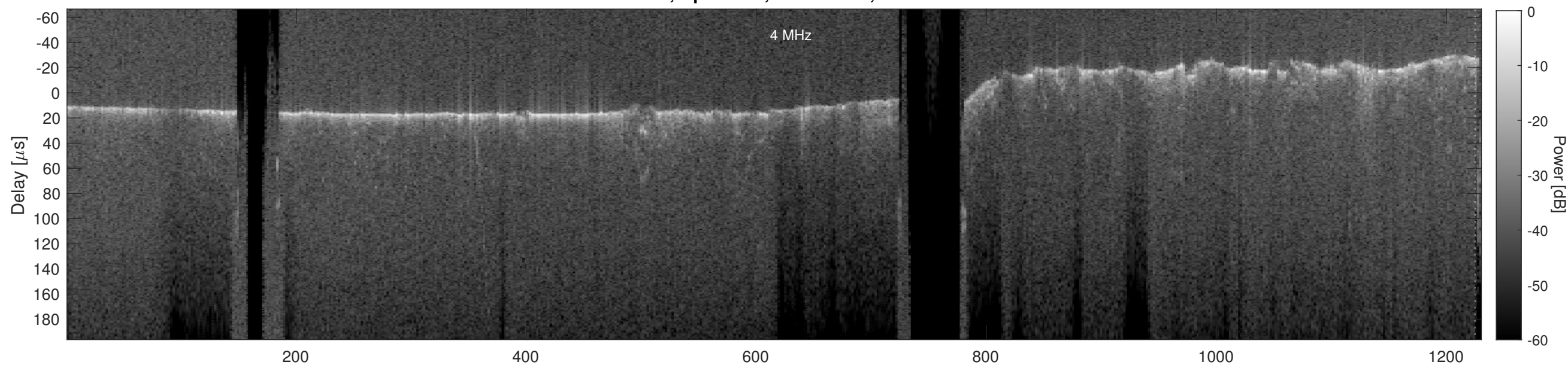
Orbit 5125, Cluttergram
