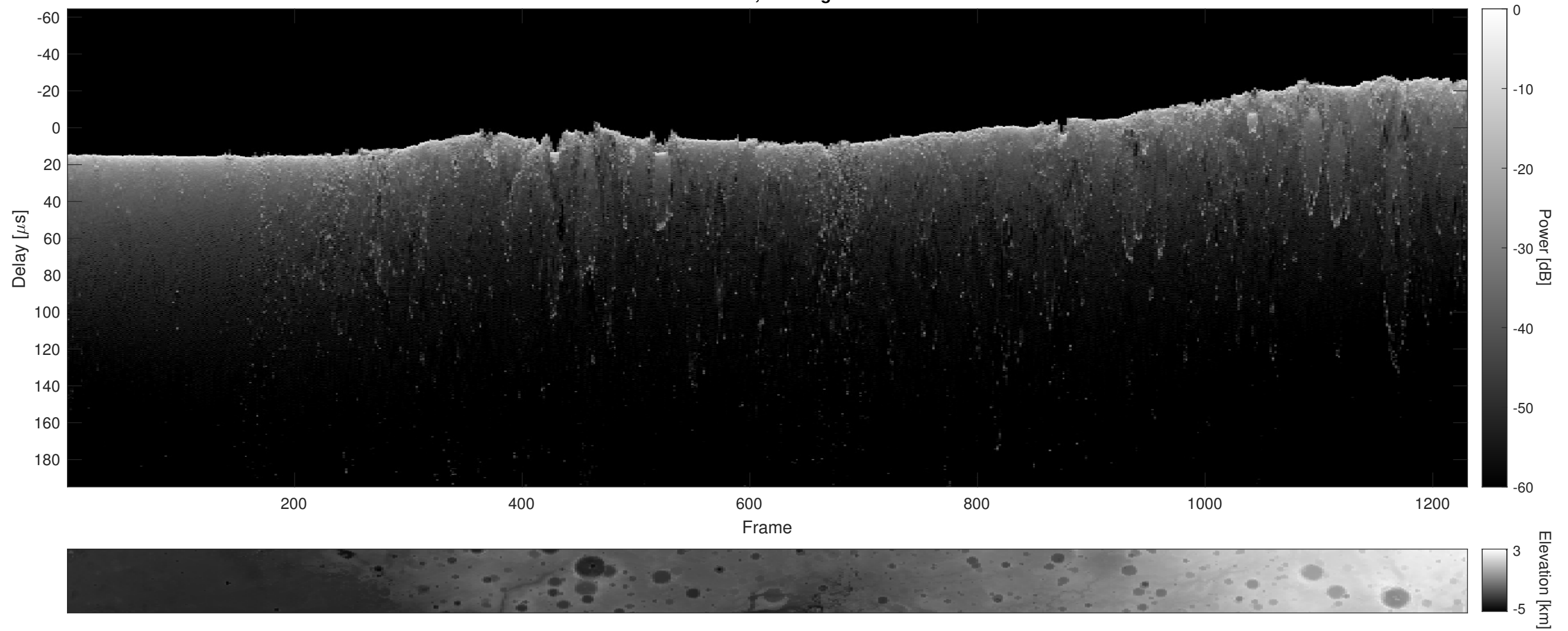
Orbit 5127, Cluttergram
