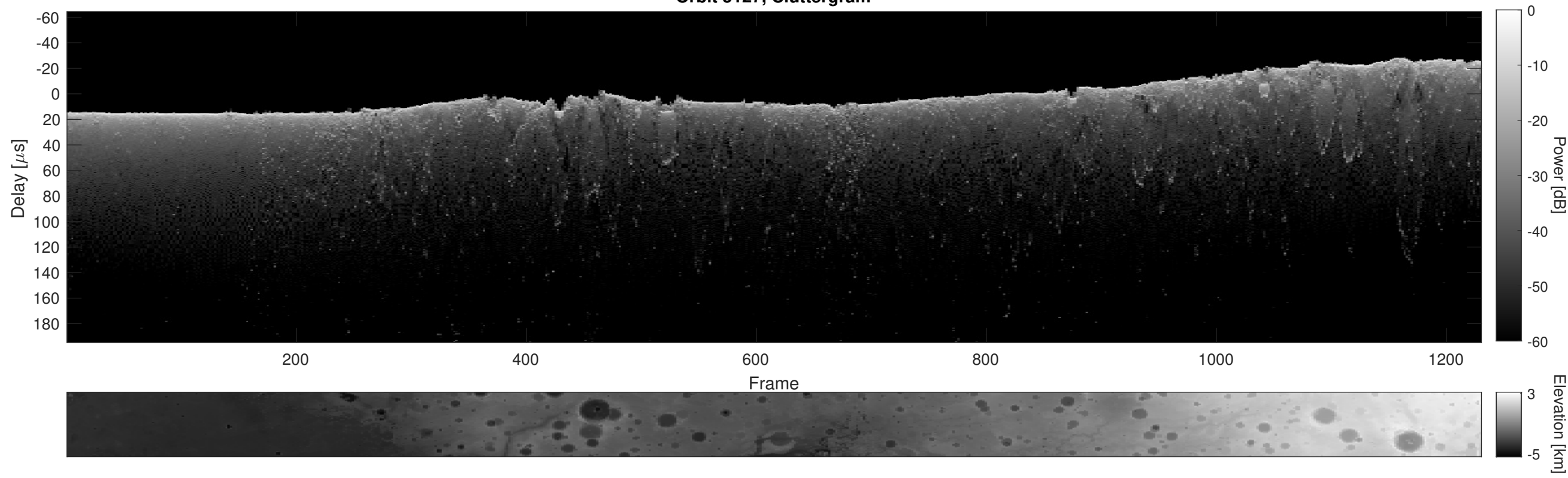
Orbit 5127, Cluttergram
