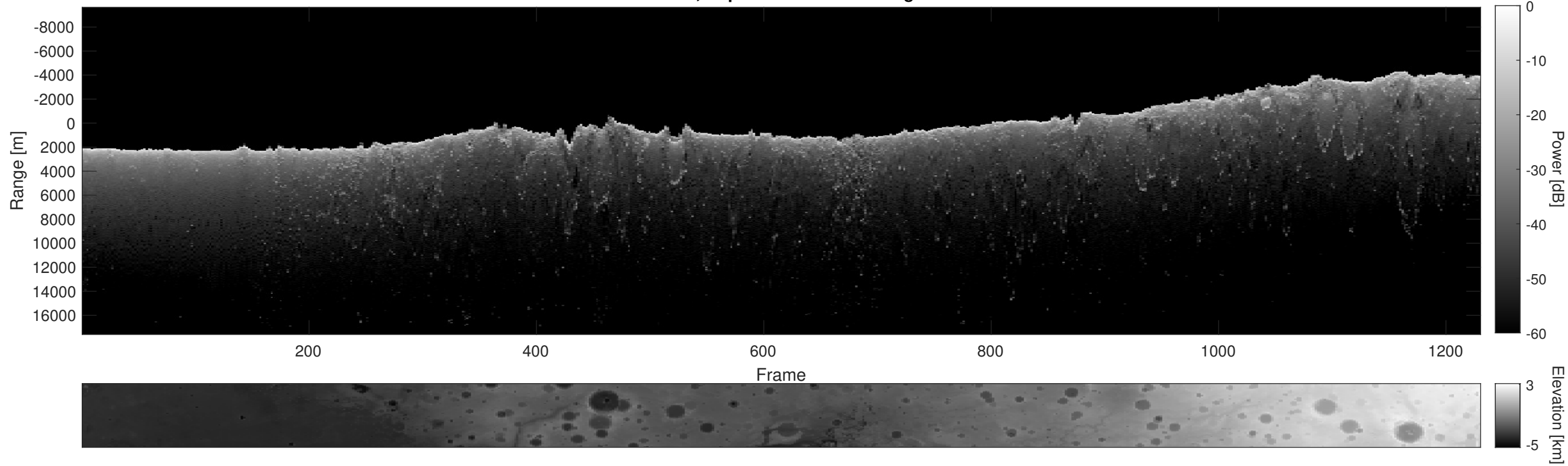
Orbit 5127, Depth-Corrected Cluttergram
