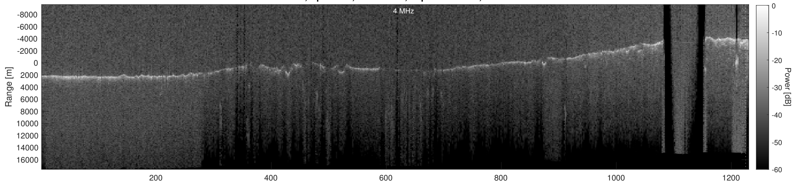
Orbit 5127, Depth-Corrected Cluttergram
