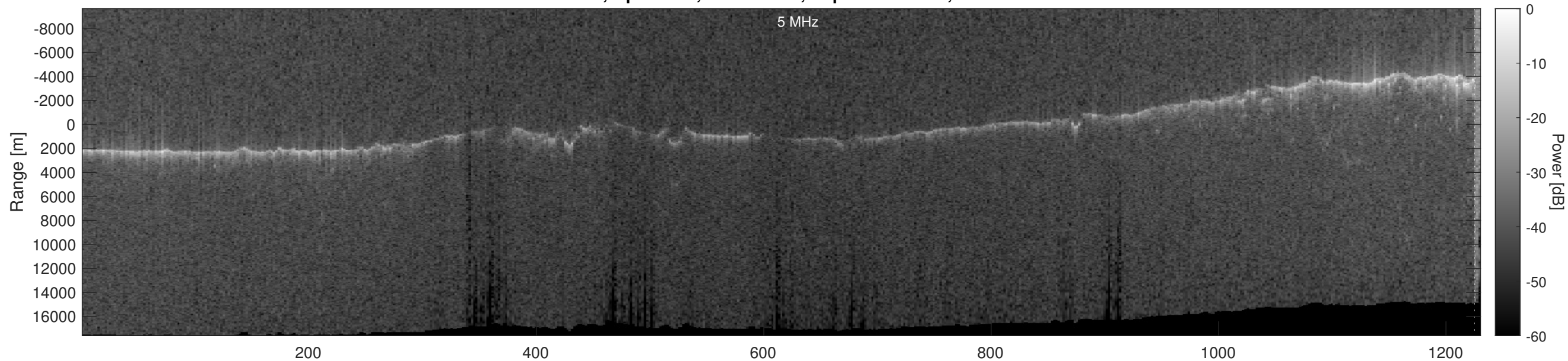
Orbit 5127, Optimized, No Window, Depth-Corrected, Channel 2
