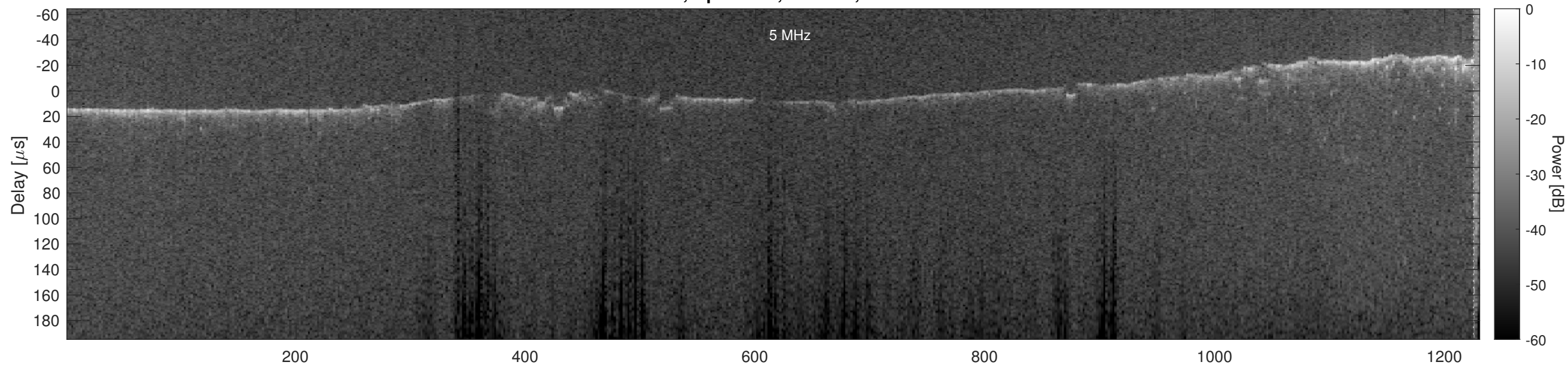
Orbit 5127, Optimized, Window, Channel 2
