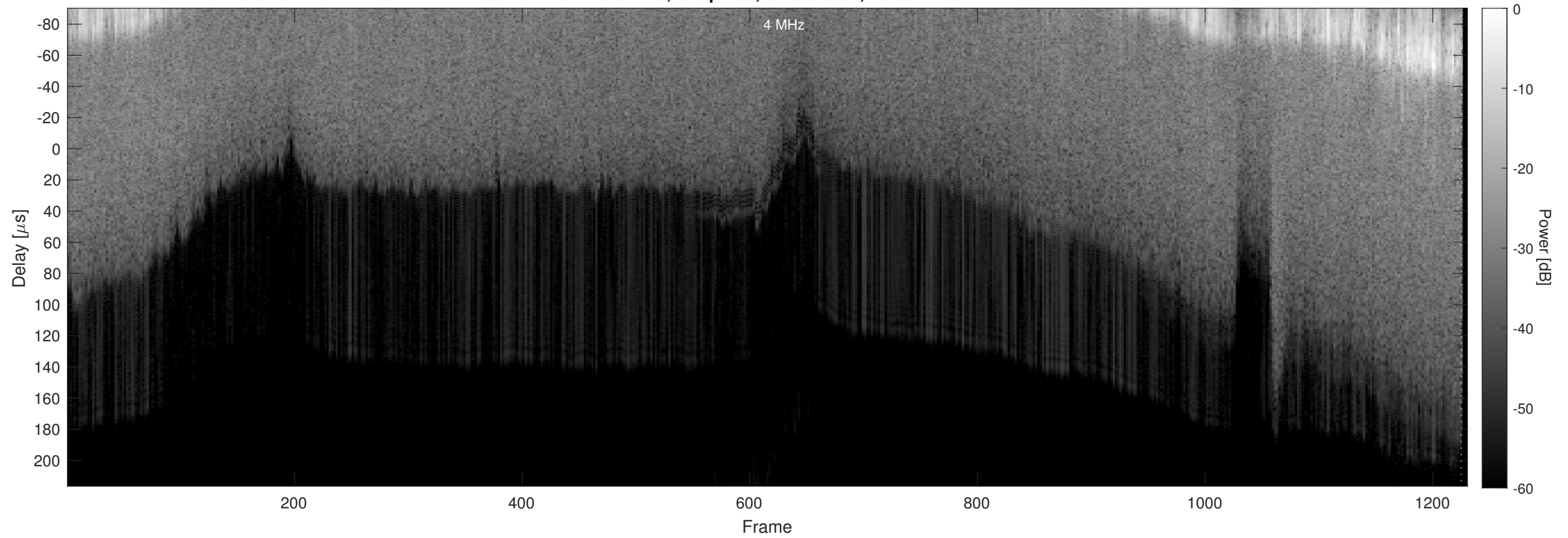
Orbit 5128, Chapman, No Window, Channel 2
