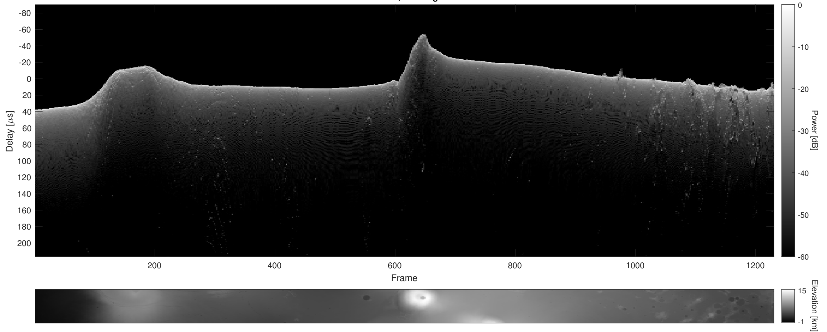
Orbit 5128, Cluttergram
