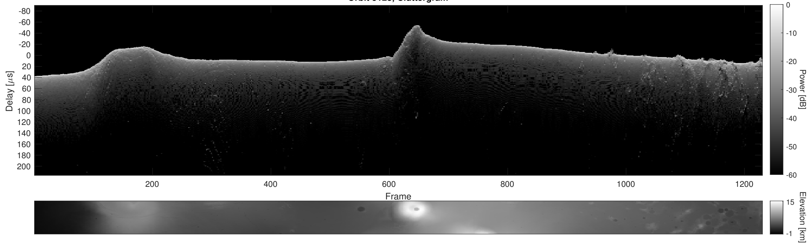
Orbit 5128, Cluttergram
