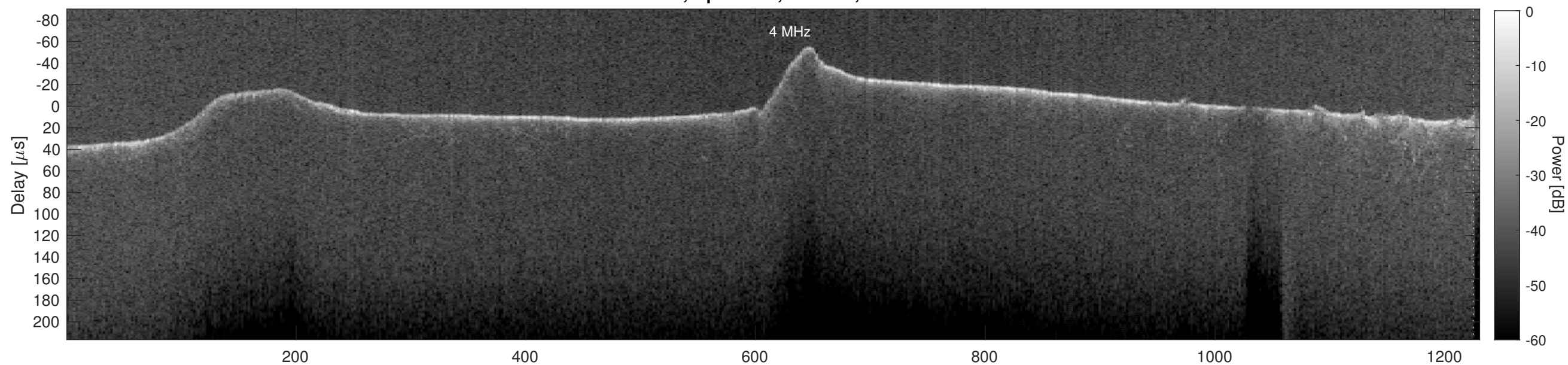
Orbit 5128, Cluttergram
