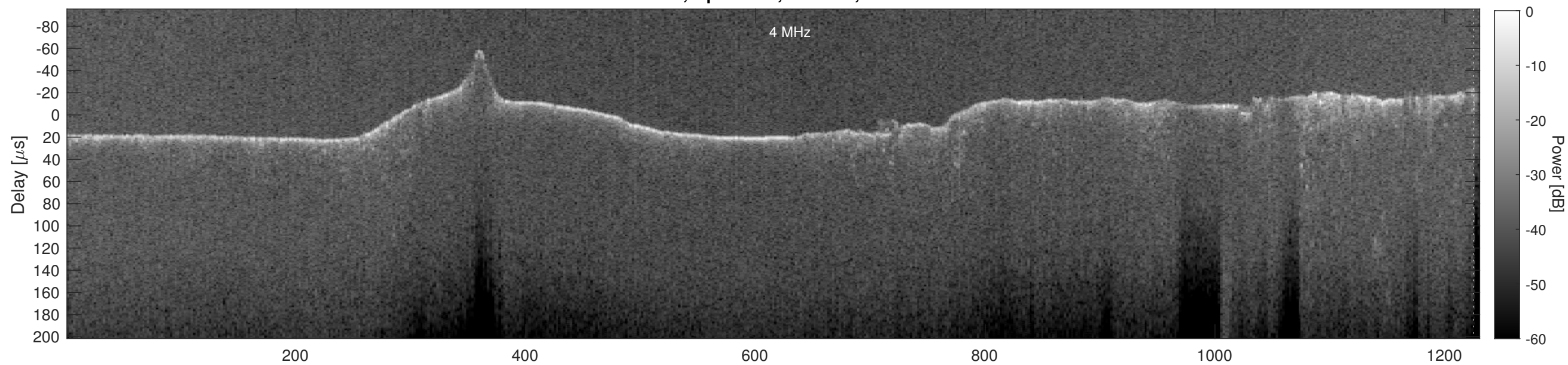
Orbit 5129, Cluttergram
