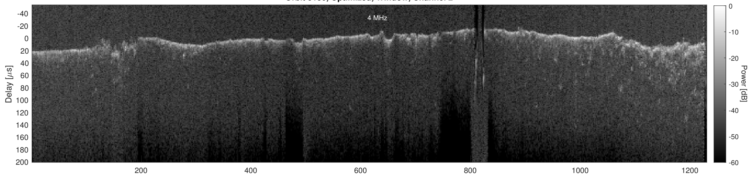
Orbit 5130, Cluttergram
