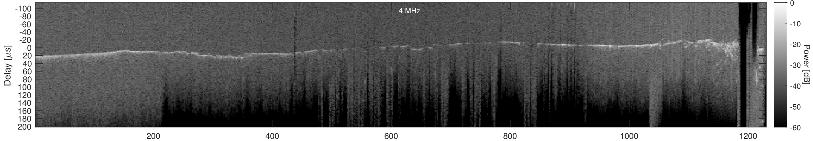
Orbit 5131, Cluttergram
