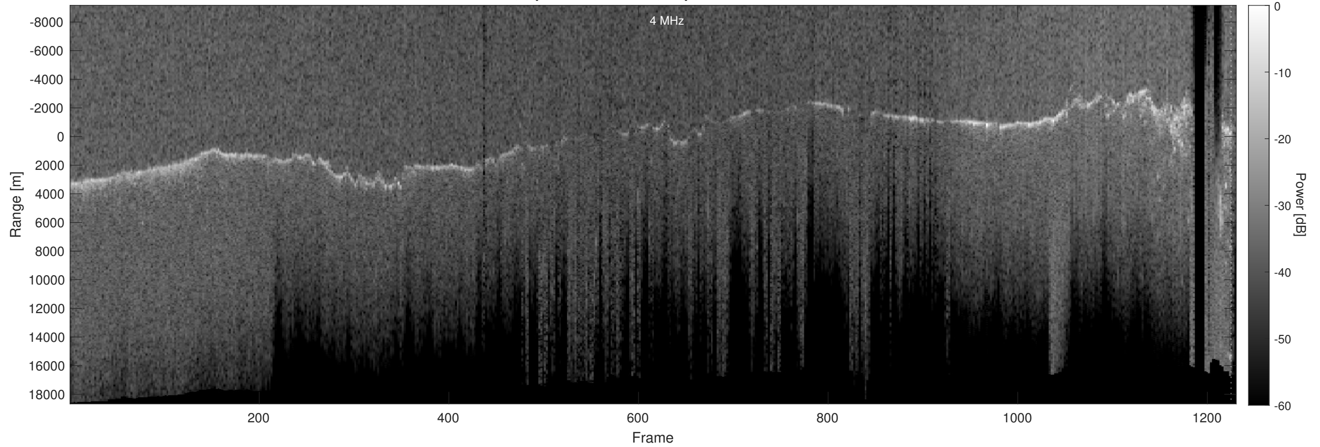
Orbit 5131, Optimized, Window, Depth-Corrected, Channel 2
