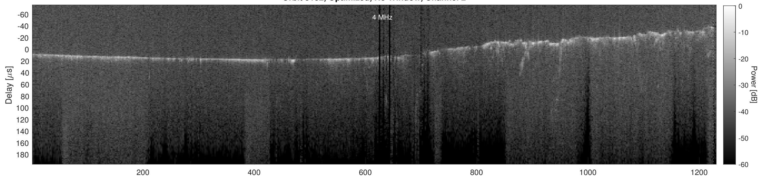
Orbit 5132, Cluttergram
