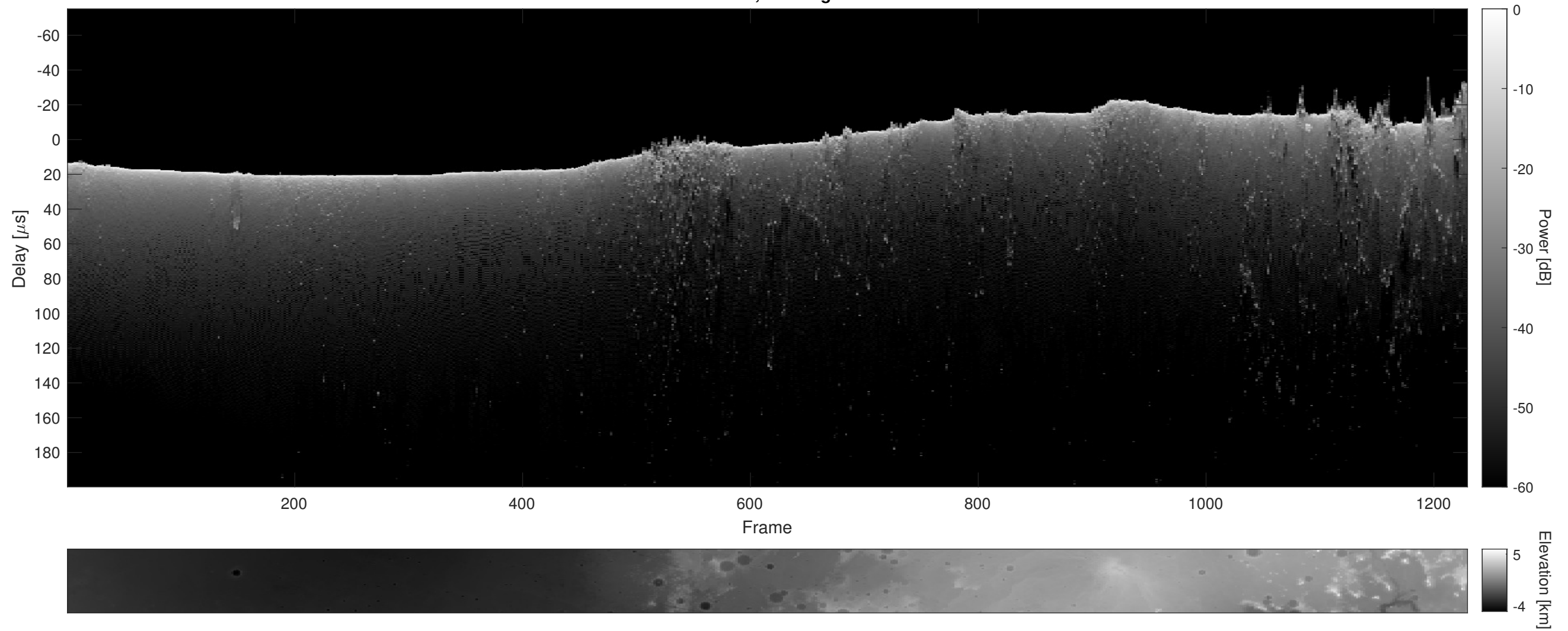
Orbit 5133, Cluttergram
