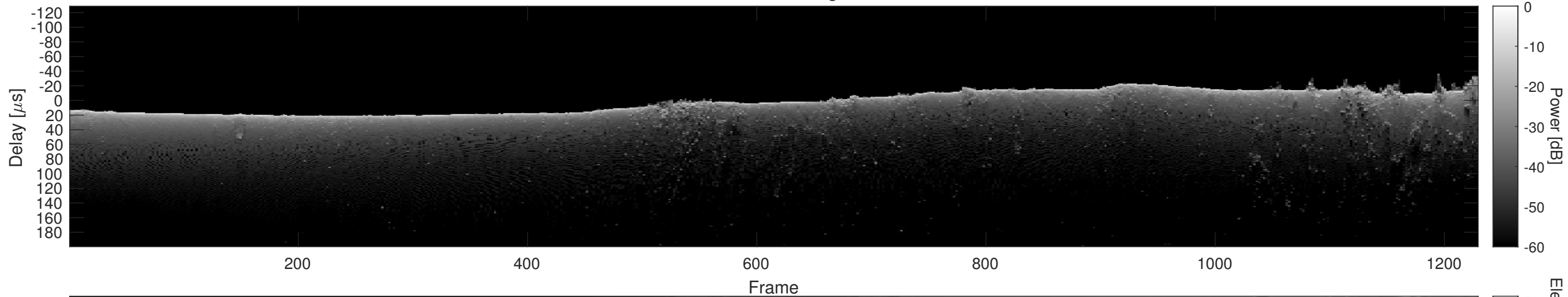
Orbit 5133, Cluttergram
