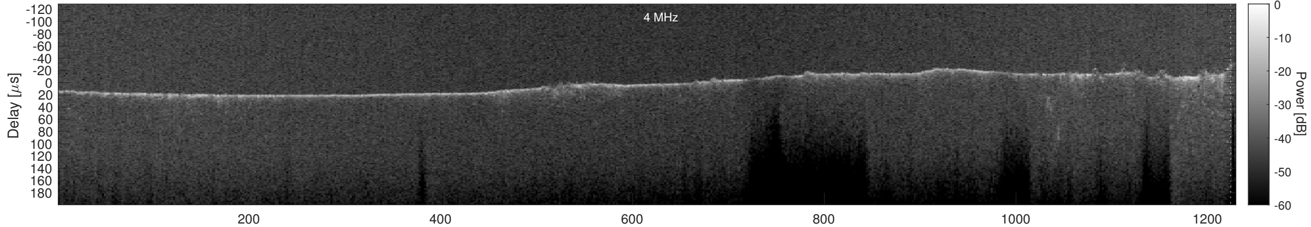
Orbit 5133, Cluttergram
