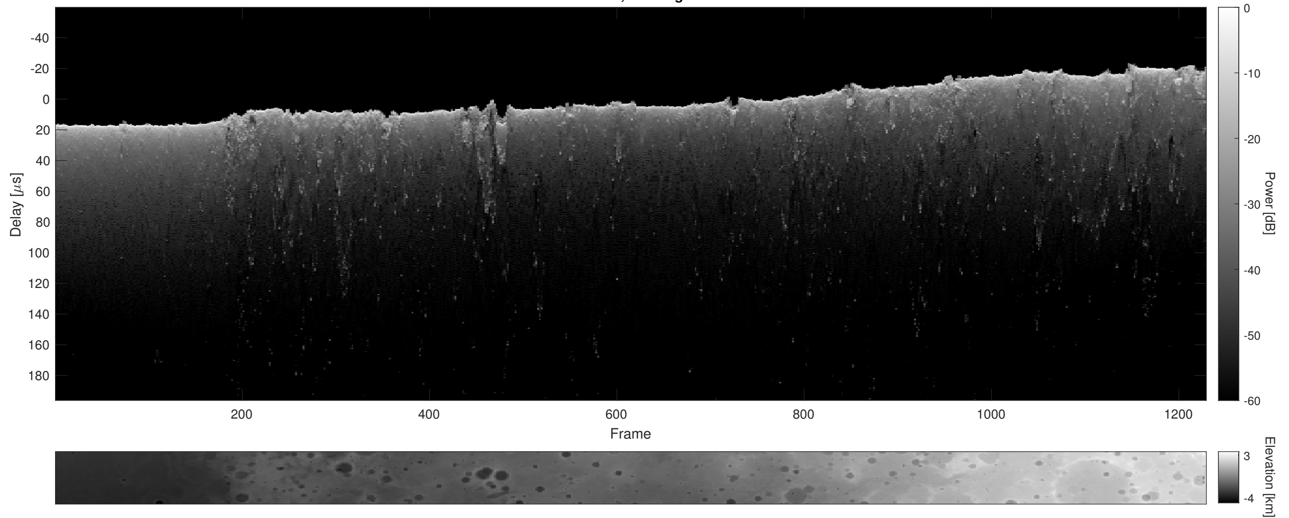
Orbit 5134, Cluttergram
