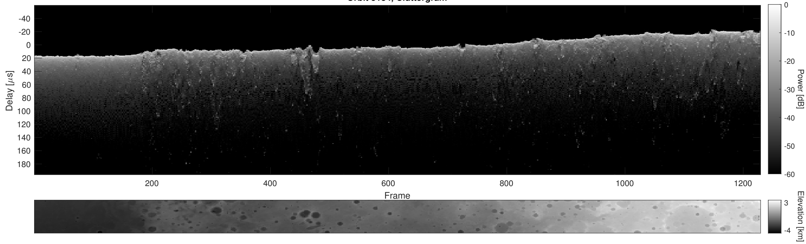
Orbit 5134, Cluttergram
