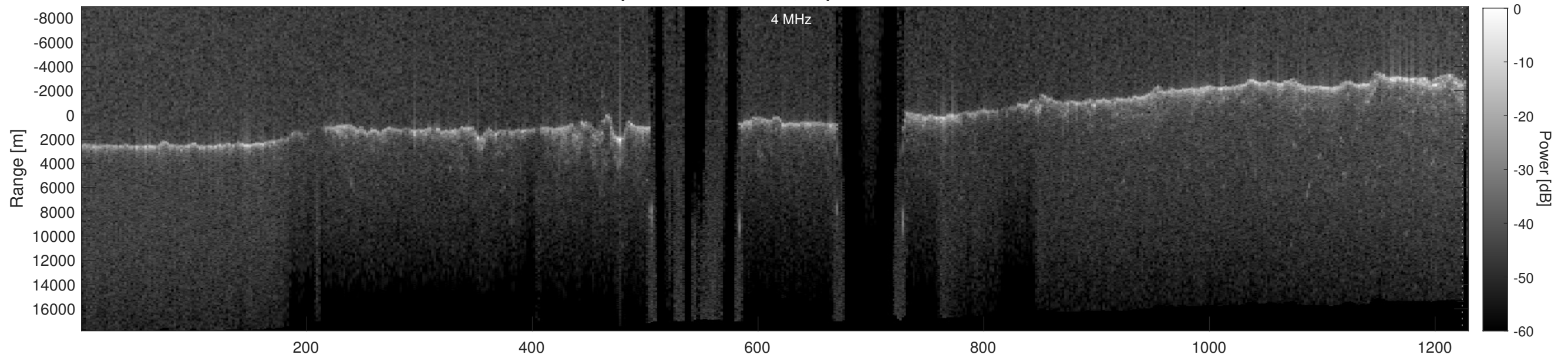
Orbit 5134, Depth-Corrected Cluttergram
