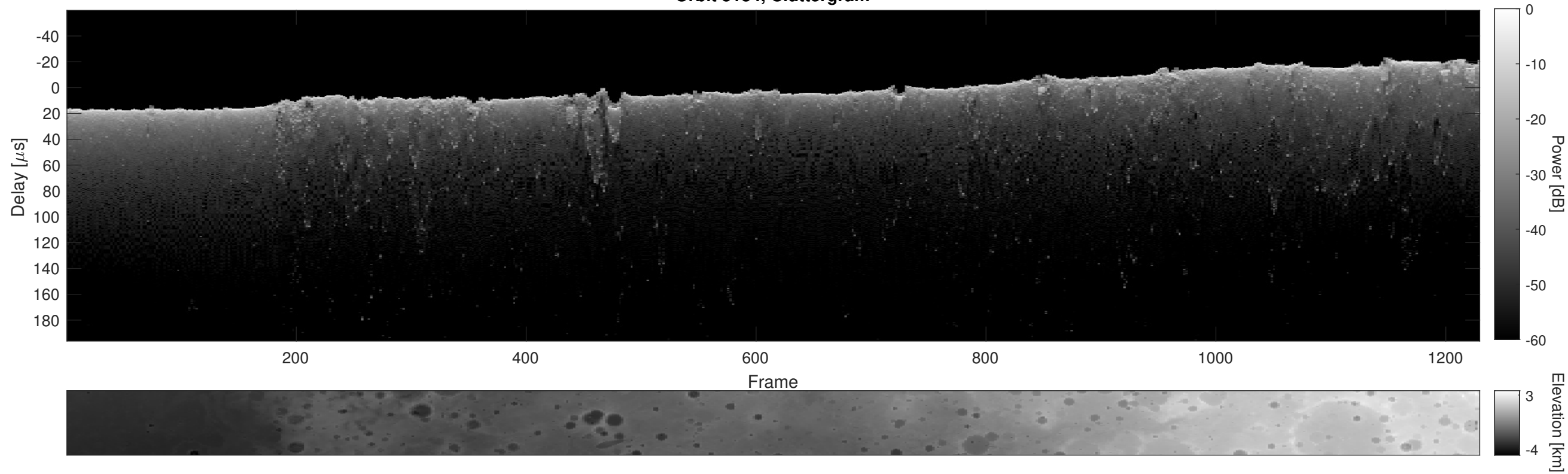
Orbit 5134, Cluttergram
