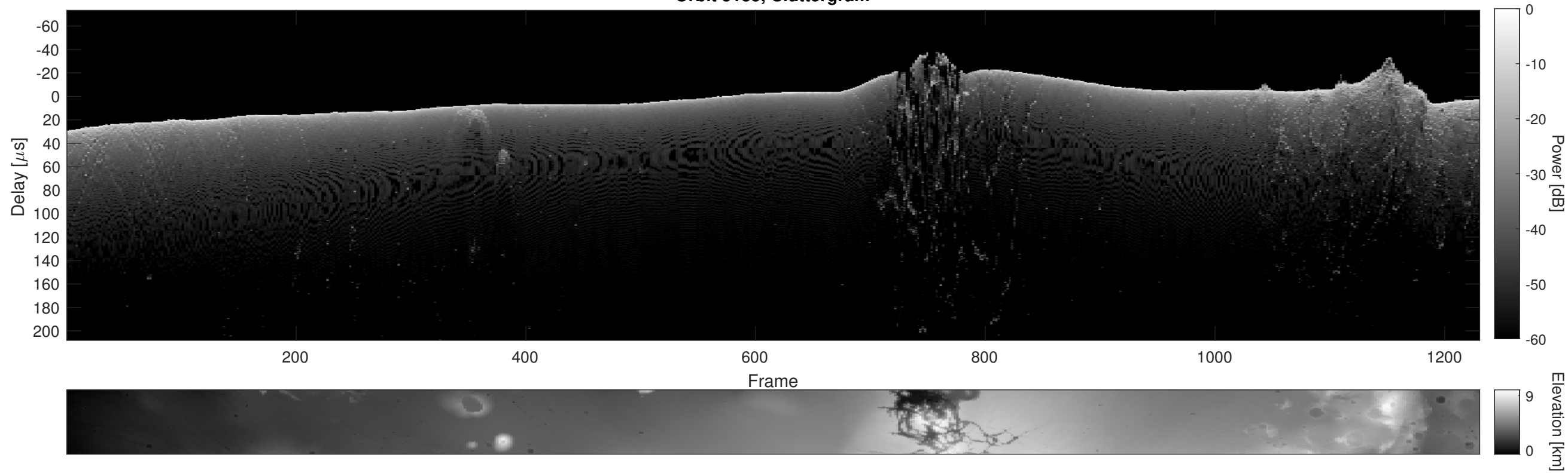
Orbit 5135, Cluttergram
