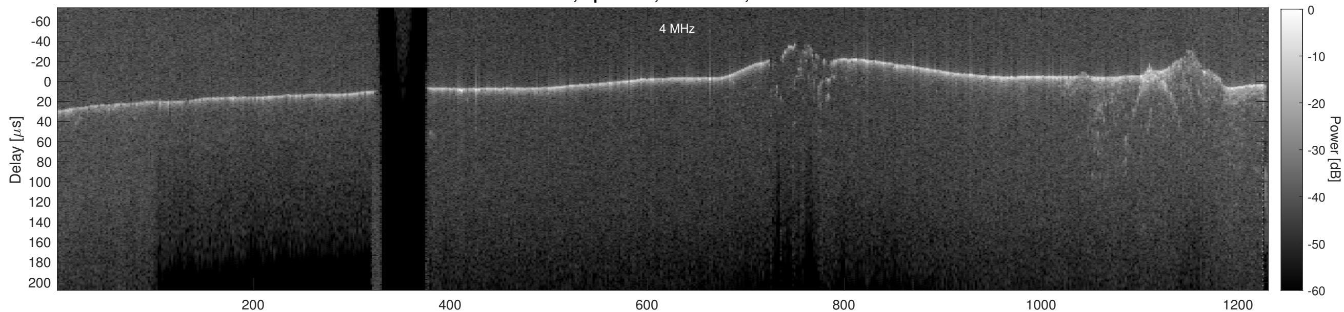
Orbit 5135, Cluttergram
